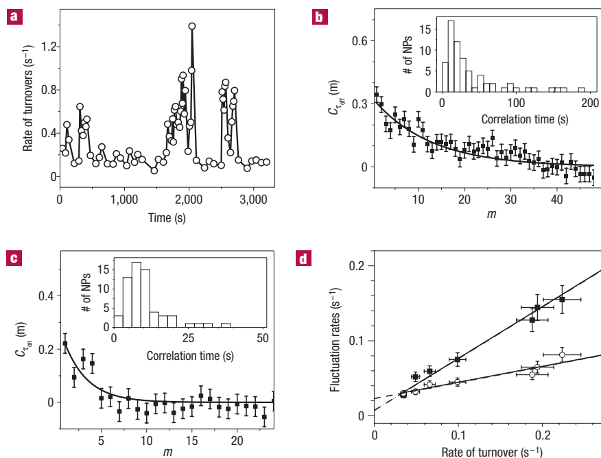
Figure 4 Single-nanoparticle catalytic dynamics. a , Trajectory of rate of turnovers for a single Au nanoparticle at 1.2 \mu\text{M} resazurin. Data points are calculated every 10 turnovers. b,c , Autocorrelation functions of \tau_{\text{off}} ( b ) and \tau_{\text{on}} ( c ) derived from the same single-turnover trajectory as that in a . Solid lines are exponential fits with decay constants of m_{\text{off}} = 12.5 \pm 2.9 and m_{\text{on}} = 2.6 \pm 0.9 turnovers. Insets: Histograms of fluctuation correlation times for \tau_{\text{off}} and \tau_{\text{on}} reactions at 1.2 \mu\text{M} resazurin. NPs: nanoparticles. d , Dependence of the activity fluctuation rate (the inverse of fluctuation correlation time) on the rate of turnovers. Circles represent the \tau_{\text{off}} reaction and squares represent the \tau_{\text{on}} reaction. Each data point is an average from >50 trajectories. Error bars are s.d. Solid lines are linear fits.
