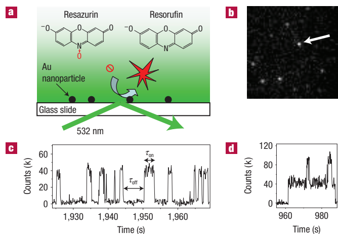
Figure 1 Single-turnover detection of single-Au-nanoparticle catalysis. a , Experimental design using total internal reflection fluorescence microscopy. b , A typical image ( \sim 18 \times 18 \mu\text{m}^2 ) of fluorescent products during catalysis taken at 100 ms per frame. The pixel size is \sim 270 nm, which results in the pixelated fluorescence spots. c , A segment of the fluorescence trajectory from the fluorescence spot marked by the arrow in b at 0.05 \mu\text{M} resazurin and 1 \text{ mM} \text{NH}_2\text{OH} . d , A segment of another fluorescence trajectory showing two on-levels at the same conditions.
