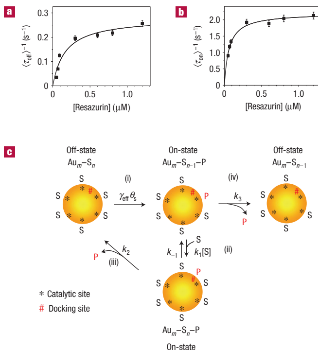
Figure 2 Kinetic mechanism of catalysis. a, b , Resazurin concentration dependence of \langle \tau_{\text{off}} \rangle^{-1} ( a ) and \langle \tau_{\text{on}} \rangle^{-1} ( b ). Each data point is an average from > 50 trajectories, each of which contains hundreds of turnovers. Solid lines are fits with equations (1) and (2) with \gamma_{\text{eff}} = 0.28 \pm 0.02 \text{ s}^{-1} , K_1 = 6 \pm 2 \mu\text{M}^{-1} , k_2 = 2.2 \pm 0.1 \text{ s}^{-1} , K_2 = 16 \pm 2 \mu\text{M}^{-1} and k_3 = 0 \pm 3 \text{ s}^{-1} . Note here the values of the kinetic parameters are the average of many nanoparticles. Errors are s.d. Note here the values of K_1 , k_2 , K_2 and k_3 represent the reactivity per site averaged over all of the sites on one nanoparticle. All error bars in the graphs are s.e.m. All experiments are in 1 \text{ mM} \text{NH}_2\text{OH} . c , Schematic diagram of the kinetic mechanism. \text{Au}_m : Au nanoparticle; S: resazurin; P: resorufin. \text{Au}_m\text{-S}_n represents a Au nanoparticle having n adsorbed substrate molecules. The fluorescence state (on or off) of the nanoparticle is indicated at each reaction stage.
