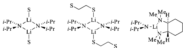
1a ; S = THF 1b ; S = n -BuOMe 1c ; S = HMPA 1d ; S = Me 2 NEt 2a ; S = OMe (DME) 2b ; S = NMe 2 (TMEDA) 3
