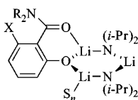
10a ; S = n -BuOMe, R = Et, X = OMe 10b ; S = HMPA, R = Et, X = OMe 10c ; S = DME, R = Me, X = F 10d ; S = \eta^1 -TMEDA, R = Me, X = OMe 10e ; S = Me 2 NEt, R = Et, X = OMe
